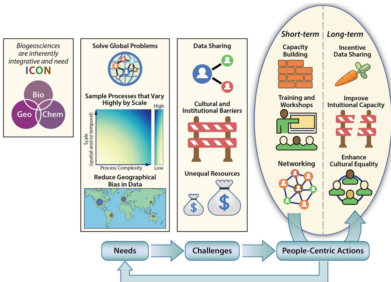
Figure 3: Conceptual overview of needs, challenges and required actions to advance biogeosciences. Geographical bias in data and unequal access to resources are identified as important issues. Source: Dwivedi et al. (2022); licensed under CC BY 4.0 .
